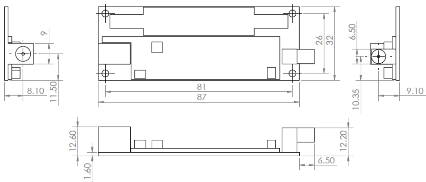
20kHz Driver (87mm x 32mm)
